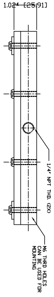
TOP VIEW WITHOUT PIPE CONNECTION
