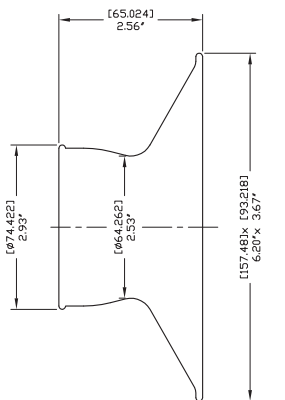
58883 - RECTANGULAR NOZZLE
