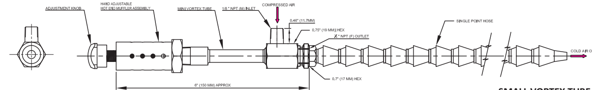
SMALL VORTEX TUBE WITH GENERATOR, HAND ADJUSTABLE HOT END MUFFLER ASSEMBLY + SINGLE POINT HOSE KIT
